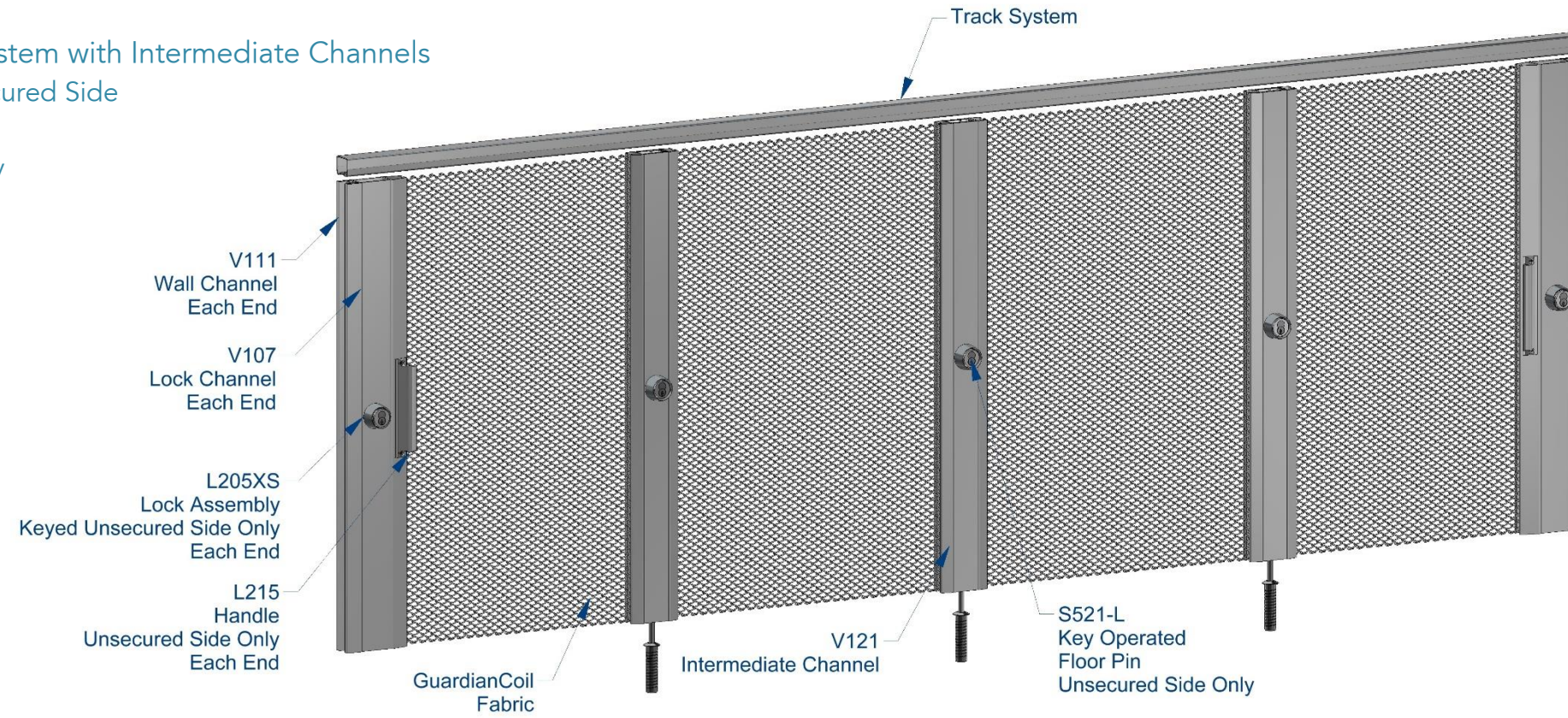
Unsecured Side
